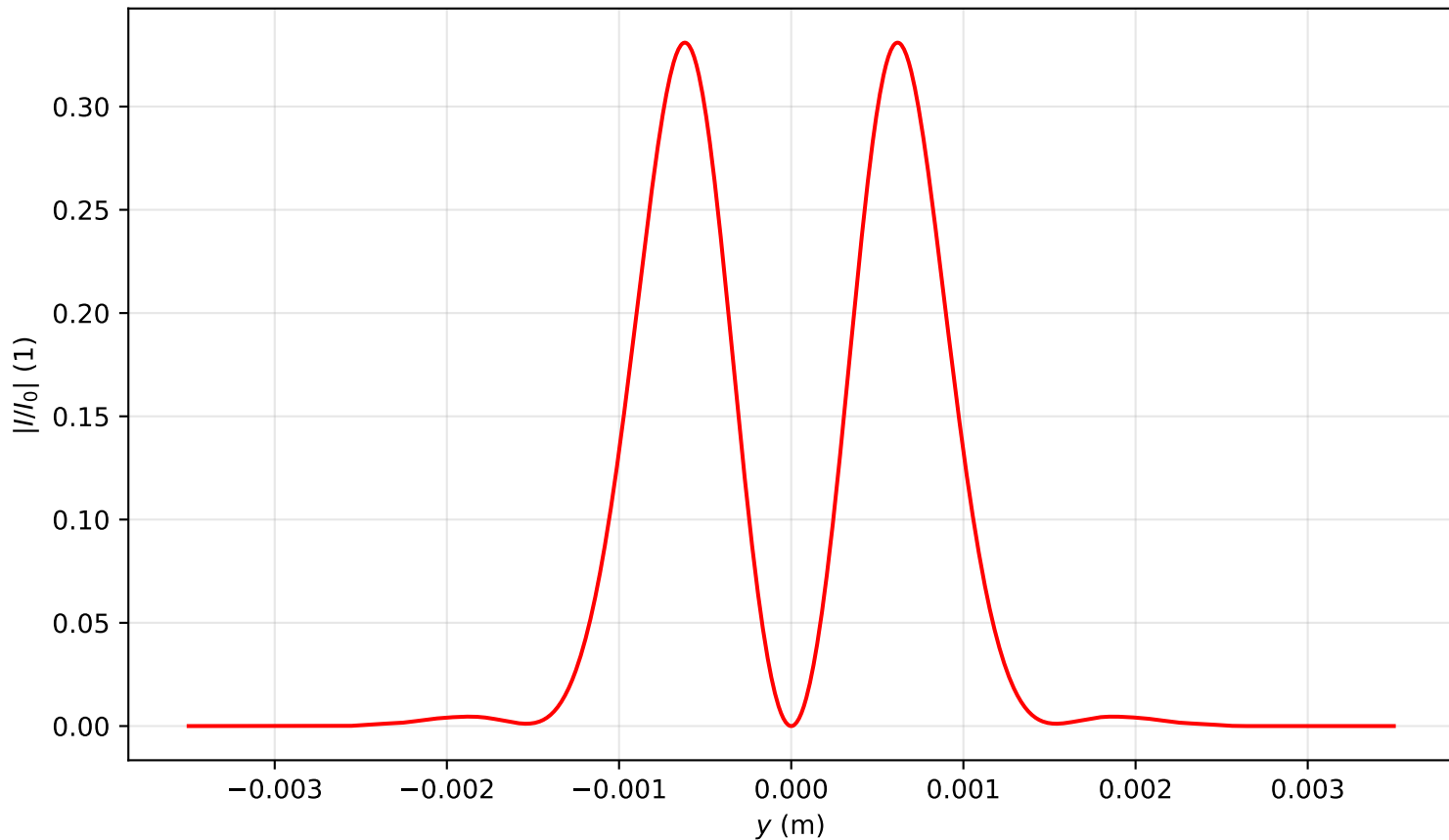
Intensity profile I(x=0, y, z=1.911)/I_0 , P_{in}=4.0P_{cr} , artificial time
